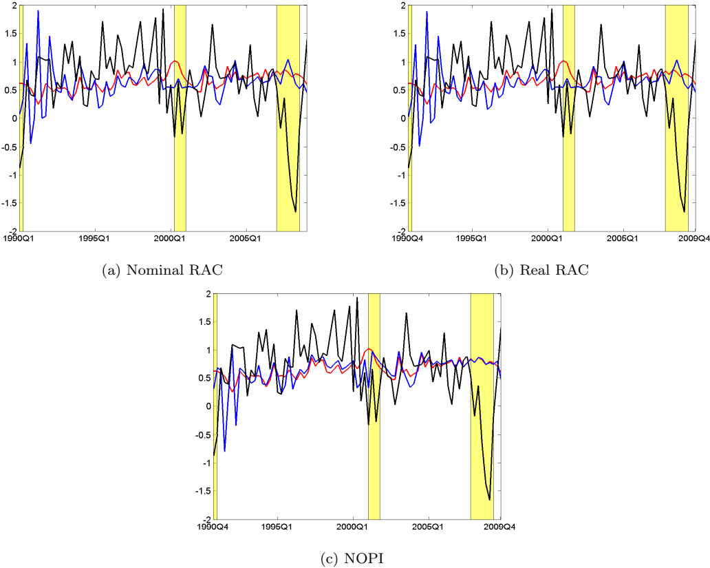
Figure A3: Real-Time Forecasts at h = 4 with Last Release Realizations
